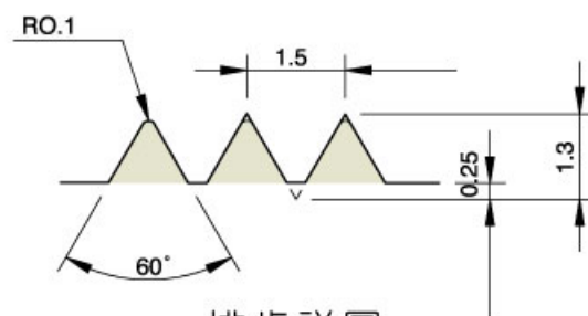
排齒詳圖 Drawing of Serration
