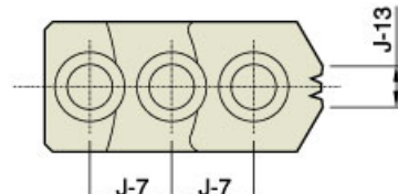
排齒詳圖 Drawing of Serration
